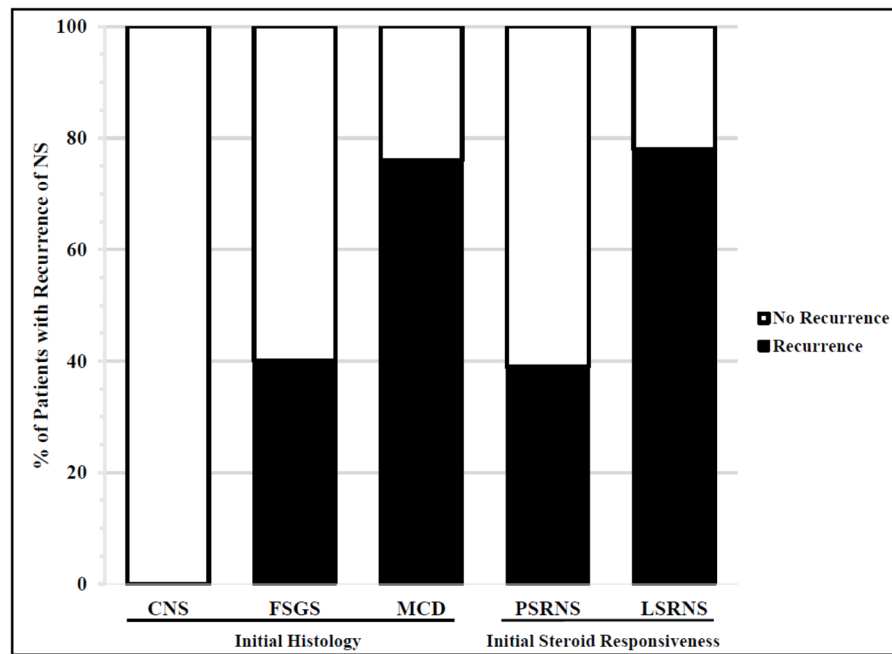
Figure 2. Proportion of patients with recurrence of nephrotic syndrome after kidney transplantation grouped by initial histology and initial steroid responsiveness. CNS congenital nephrotic syndrome, FSGS focal segmental glomerulosclerosis, MCD minimal change disease, PSRNS Primary steroid-resistant nephrotic syndrome, LSRNS Late steroid-resistant nephrotic syndrome. Note that all CNS were due to single gene mutation (monogenic NS).
