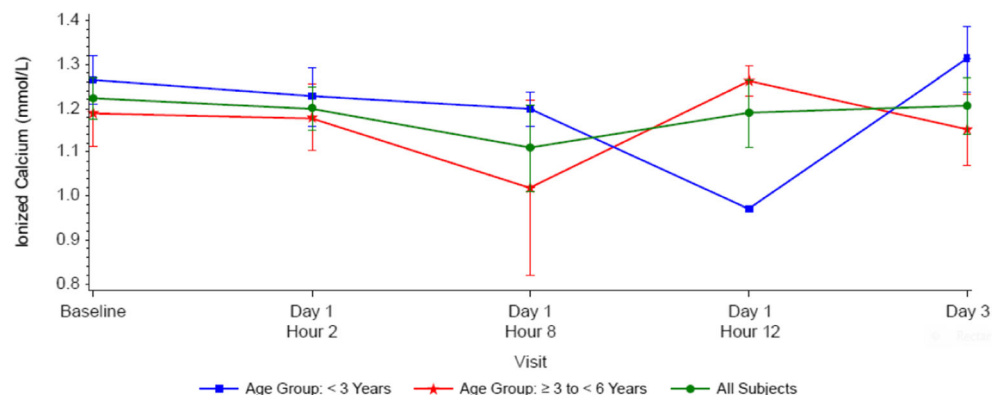
Fig. 6 Mean (SE) ionized calcium (cCa) concentrations over time by age group (< 3 years ( n = 4 ); age \geq 3 years < 6 years ( n = 8 ); all subjects ( n = 12 ))
